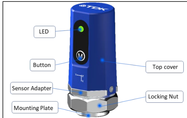
Figure 1: Sensor exterior
