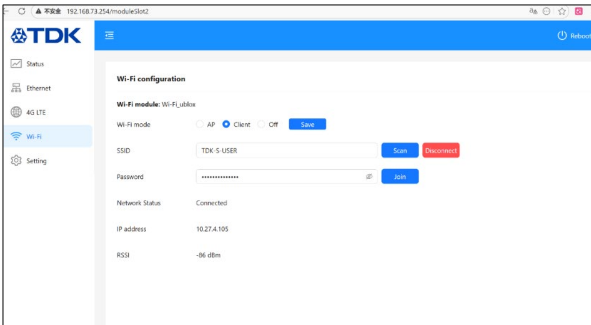
Figure 14: Gateway as client mode
