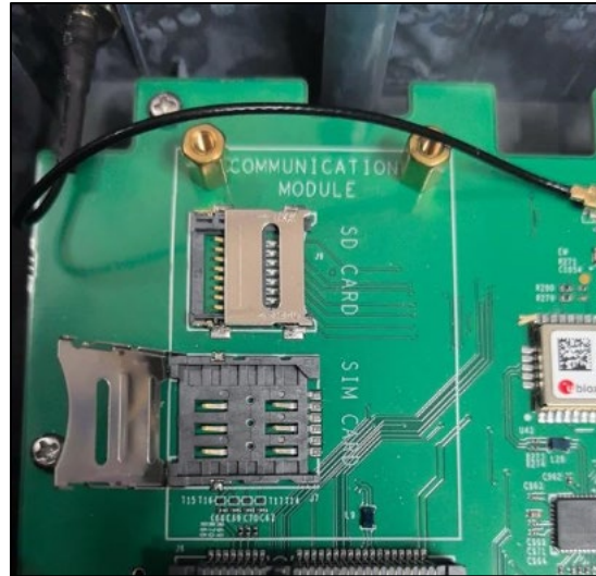
Figure 16: Gateway SIM card holder
